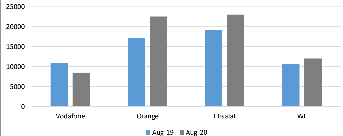
Uplink Throughput (Kbps) Alexandria Region
