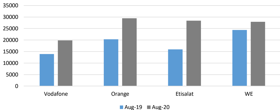
Downlink Throughput (Kbps) Delta Region
